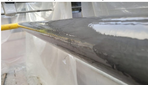
Rust, grime and paint were ground off the pipe and the three metre section coated in Liquid Metal
